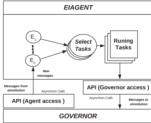
Fig. 2. EIAgent's abstract architecture
