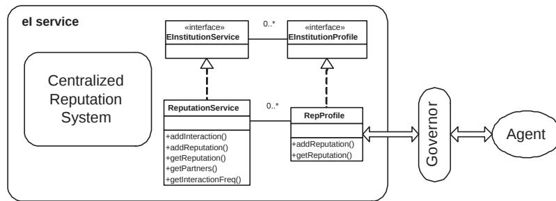
Fig. 1. Centralized reputation system as an eI service
